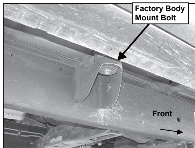
(Fig 2) Passenger/right center body mount
