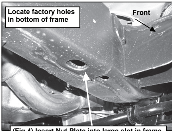
(Fig 4) Insert Nut Plate into large slot in frame
