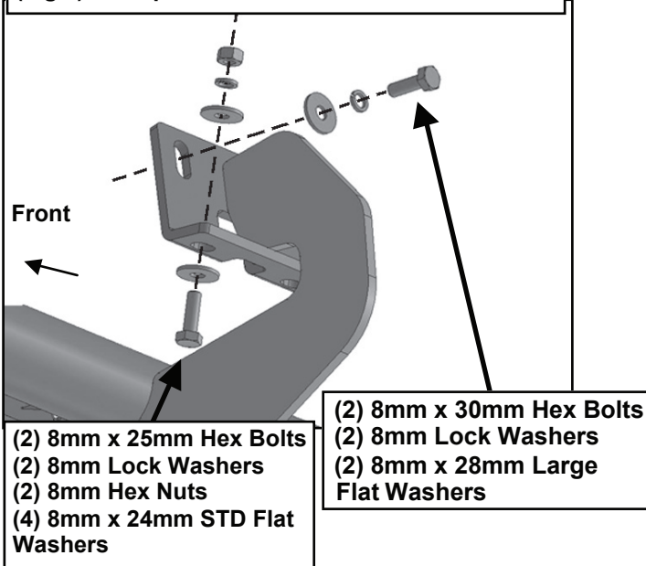
(Fig 5) Example of front/rear Bracket installation
