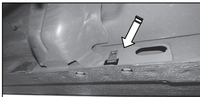
(Fig 3) Passenger/right center mounting location. NOTE: Requires (1) 8mm Clip Nut only (arrow)
