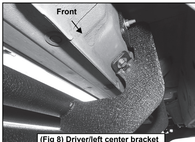
(Fig 8) Driver/left center bracket installed (early model pictured)
