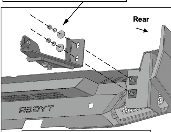
(Fig 23) Remove Screens for accessory light installation (lights not included)
