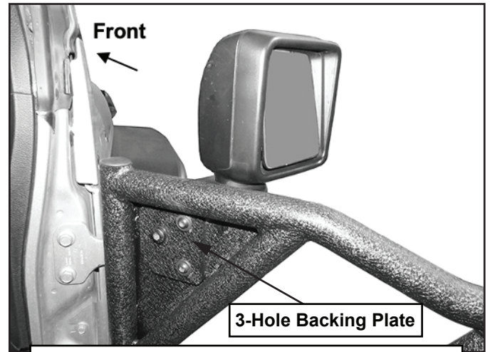
(Fig 11) Passenger/right mirror attached to Door
