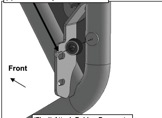
(Fig 4) Attach Rubber Bumper to mount on back of Tube Door
