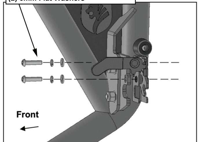
(Fig 6) Attach passenger/right Latch to Bracket on Door.
