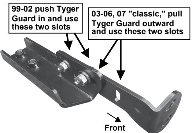
(Fig 3) driver/left Tube to Frame Bracket Assembly
