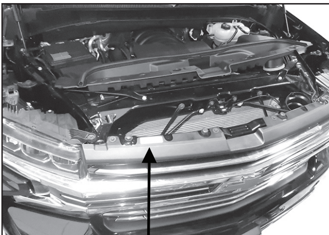
(Fig 5) Remove cover and screws attaching grille
