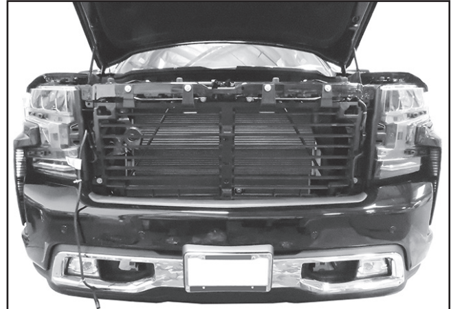
(Fig 6) Firmly pull grille straight out from vehicle
