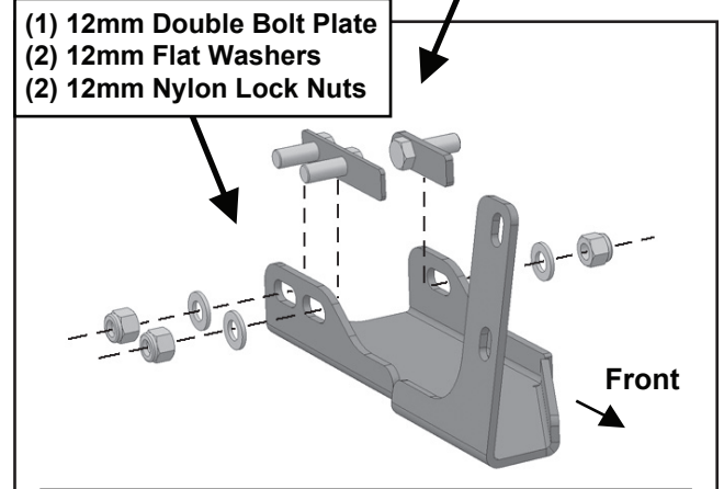
(Fig 12) Passenger/Right side Bracket illustrated
