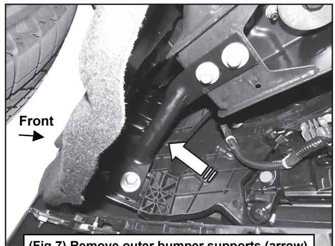
(Fig 7) Remove outer bumper supports (arrow)
