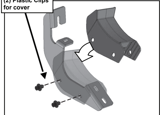
(Fig 5) Passenger front Bracket cover installation
