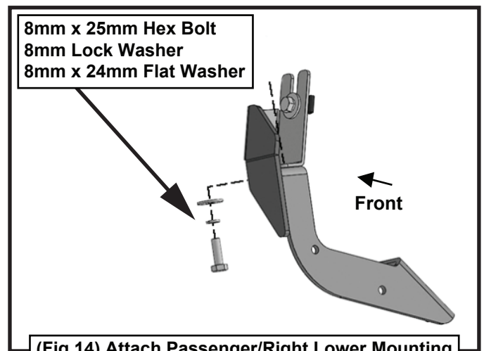
(Fig 14) Attach Passenger/Right Lower Mounting Bracket to the upper Mounting Bracket
