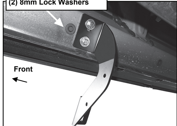
(Fig 7) Passenger side center Bracket installation
