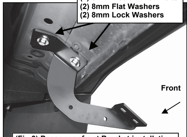
(Fig 3) Passenger front Bracket installation
