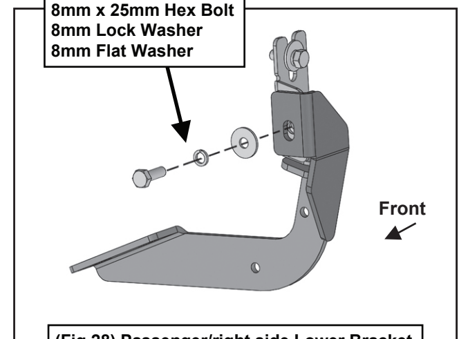
(Fig 28) Passenger/right side Lower Bracket attached to Upper Bracket
