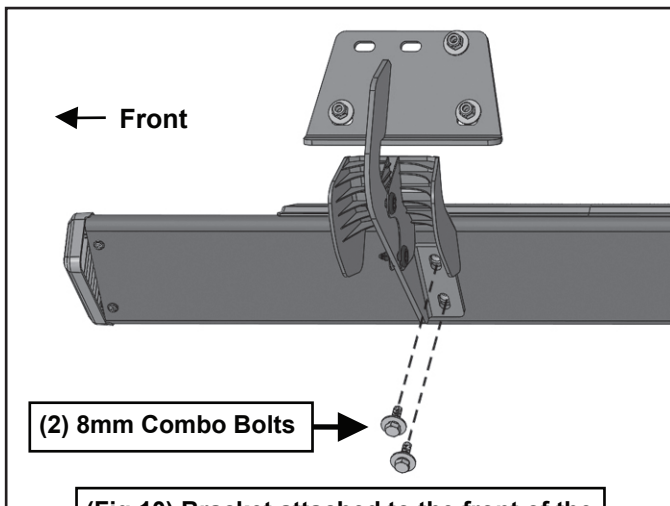
(Fig 10) Bracket attached to the front of the Passenger/right Sidebar
