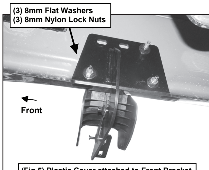
(Fig 5) Plastic Cover attached to Front Bracket
