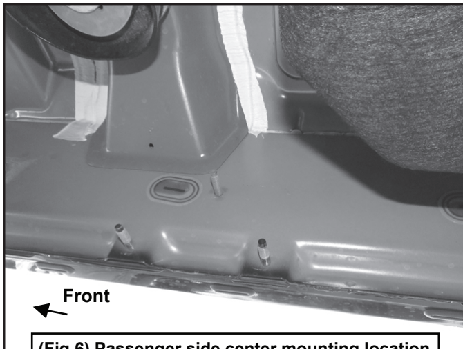
(Fig 6) Passenger side center mounting location
