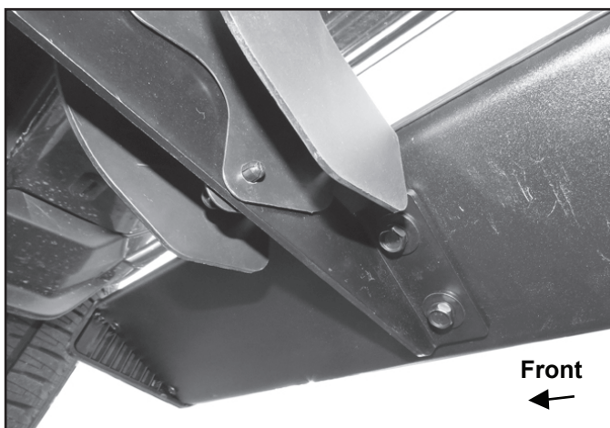
(Fig 11) Passenger/right Sidebar attached to Mounting Bracket at the front location
