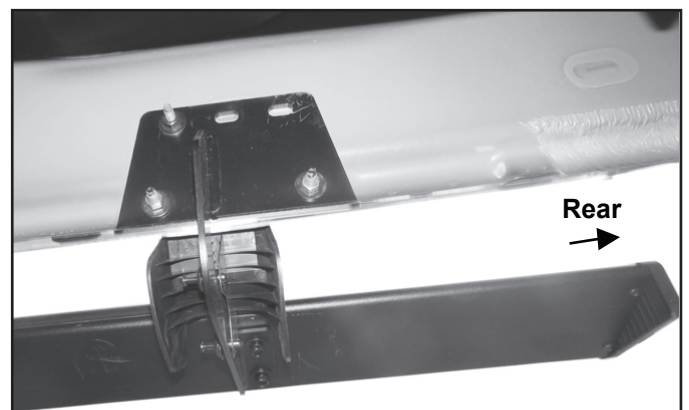
(Fig 13) Passenger/right Sidebar attached to Mounting Bracket at the rear location
