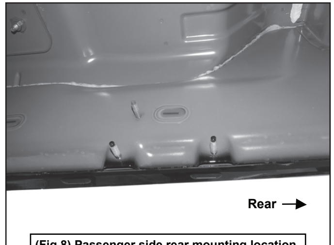
(Fig 8) Passenger side rear mounting location
