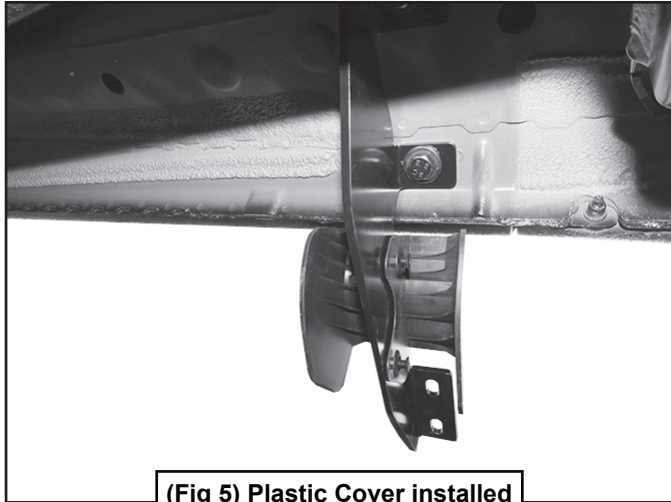
(Fig 5) Plastic Cover installed
