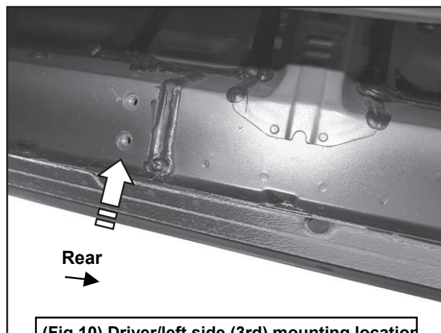
(Fig 10) Driver/left side (3rd) mounting location
