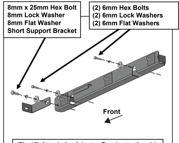
(Fig 15) Attach the Adaptor Bracket to the side of the bed (For vehicles without bedrails)
