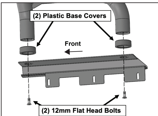
(Fig 6) Passenger/Right Base Bracket installation
