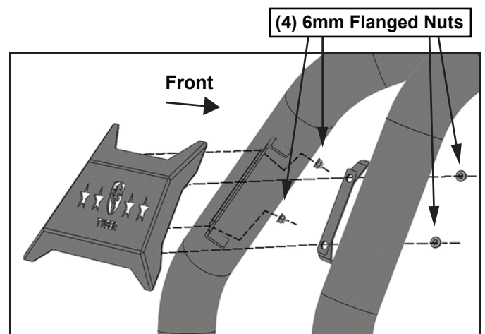
(Fig 7) Passenger/Right Decorative Plate installation
