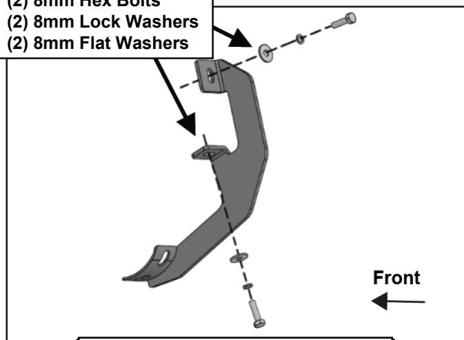
(Fig 4) Mounting Bracket illustration
