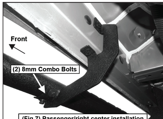
(Fig 7) Passenger/right center installation
