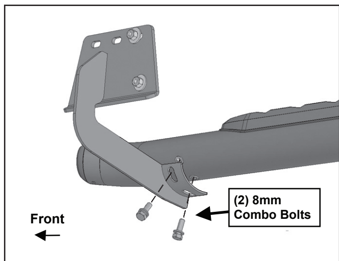
(Fig 9) Attach Passenger/Right Sidebar P to front Bracket
