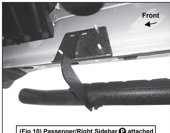
(Fig 10) Passenger/Right Sidebar P attached to front Bracket
