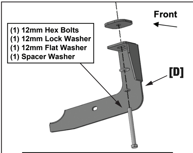
(Fig 3) Attach the Passenger/Right Front Mounting Bracket [D] to the front location
