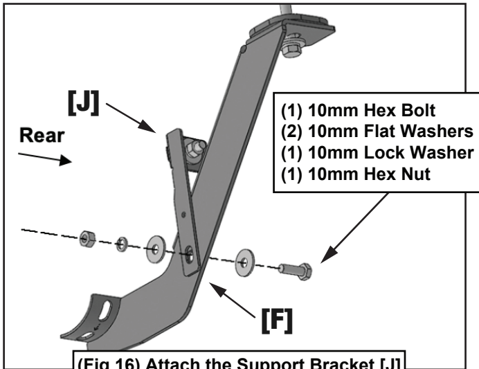
(Fig 16) Attach the Support Bracket [J] to the Mounting Bracket [F]
