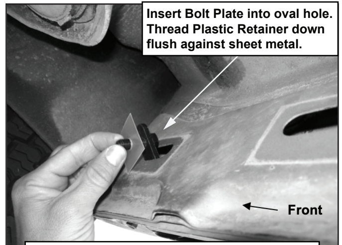
(Fig 5) Insert Bolt Plate into hole in body panel
