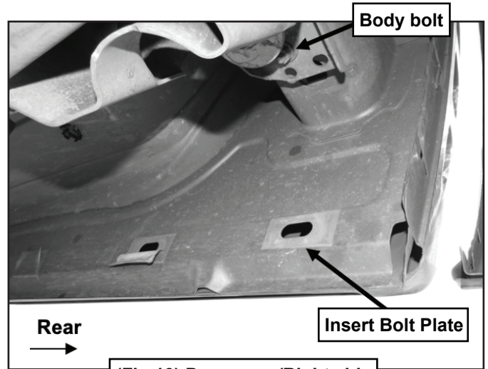
(Fig 13) Passenger/Right side Rear mounting location
