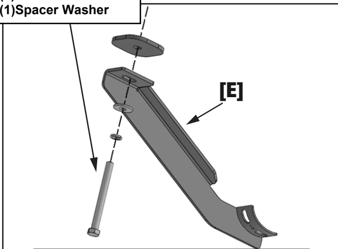
(Fig 12) Attach the Passenger/Right Center Mounting Bracket [E] to the center location
