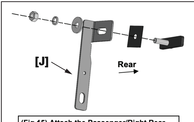
(Fig 15) Attach the Passenger/Right Rear Support Bracket (Short) [J] to the Bolt Plate
