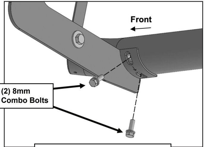
(Fig 17) Attach the Passenger/Right Sidebar to the Mounting Brackets
