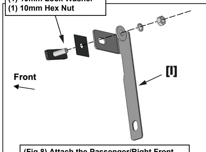
(Fig 8) Attach the Passenger/Right Front Support Bracket (Long) [I] to the pinch weld
