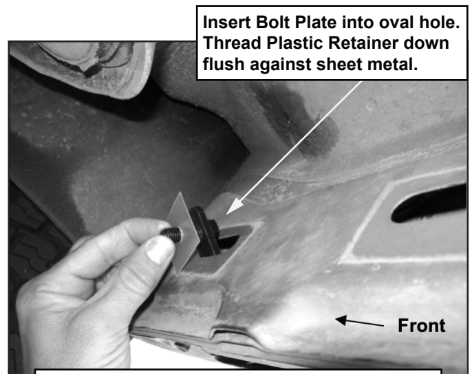
(Fig 5) Insert Bolt Plate into hole in body panel
