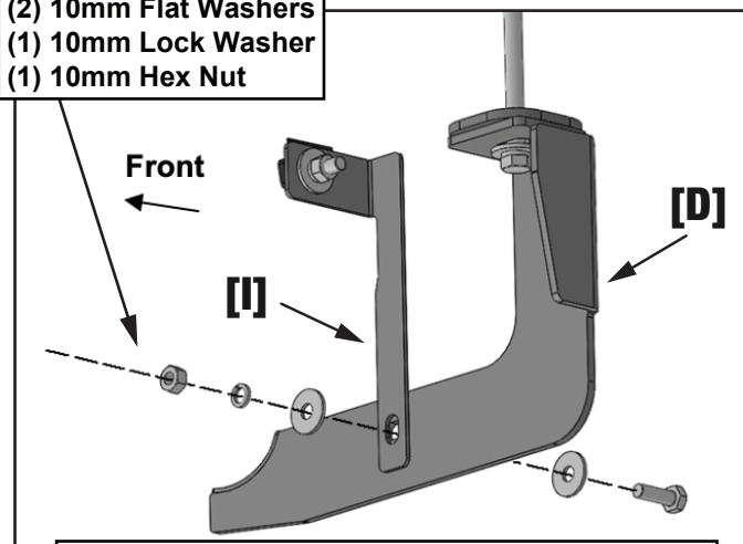
(Fig 9) Attach the Passenger/Right Front Support Bracket [I] to the Mounting Bracket [D]
