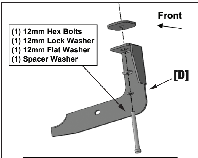
(Fig 3) Attach the Passenger/Right Front Mounting Bracket [D] to the front location
