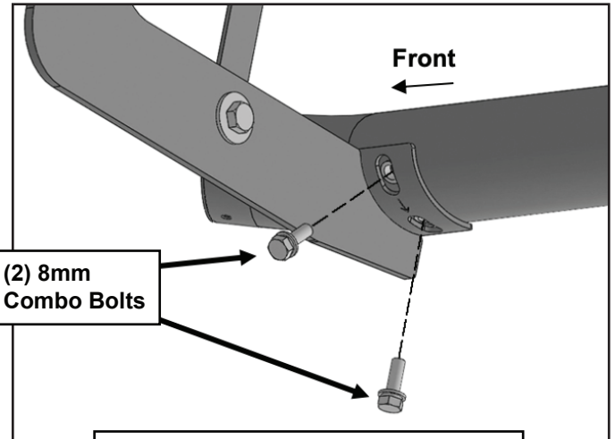
(Fig 17) Attach the Passenger/Right Tyger Rider to the Mounting Brackets
