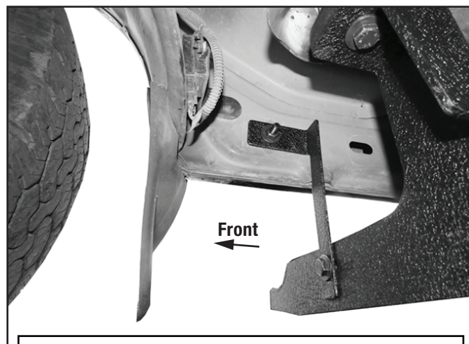
(Fig 10) Passenger/Right Front Support Bracket [I] attached to the Mounting Bracket [D]
