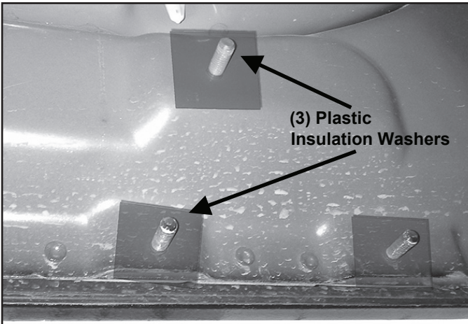
(Fig 3) Thread Plastic Washers onto all mounting studs
