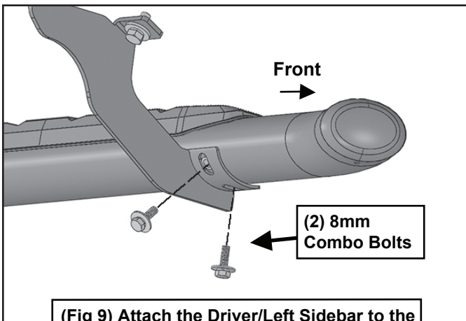
(Fig 9) Attach the Driver/Left Sidebar to the Mounting Brackets
