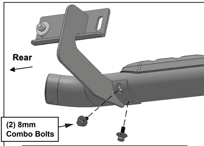
(Fig 13) 3-door model, driver/left side only. Attach Tyger Rider to the Rear Bracket
