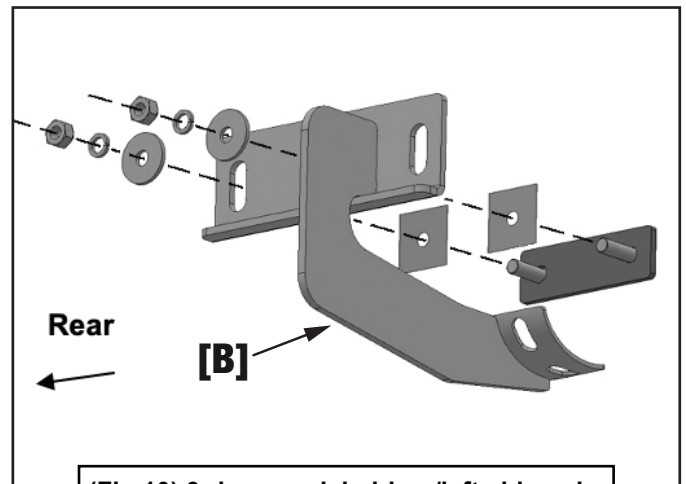
(Fig 10) 3-door model, driver/left side only. Attach the Driver/Left Rear Bracket [B] to the Small 10mm Bolt Plate. Use the center and rear slots only.
