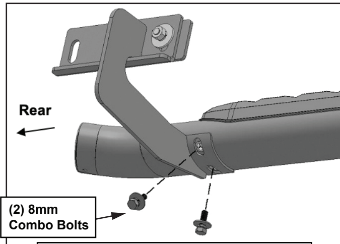
(Fig 12) 4-door model, driver/left side only. Attach Tyger Rider to the Rear Bracket
