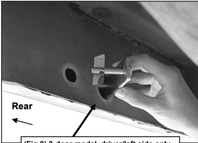
(Fig 8) 3-door model, driver/left side only. Insert the Small Double Bolt Plate into the large hole and back out the smaller hole. Tighten the Plastic Retainer down to the body panel to hold the Bolt Plate in place
