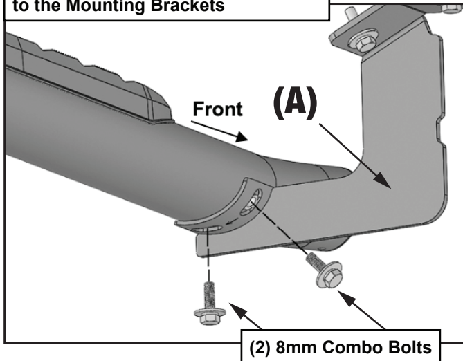
(Fig 7) Attach the Driver/Left Sidebar to the Mounting Brackets
