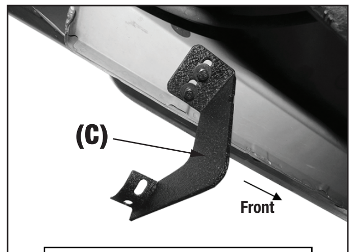
(Fig 6) Driver/Left Rear Mounting Bracket (C) attached to the front location
