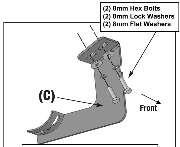
(Fig 5) Attach the Driver/Left Rear Mounting Bracket (C) to the front location
