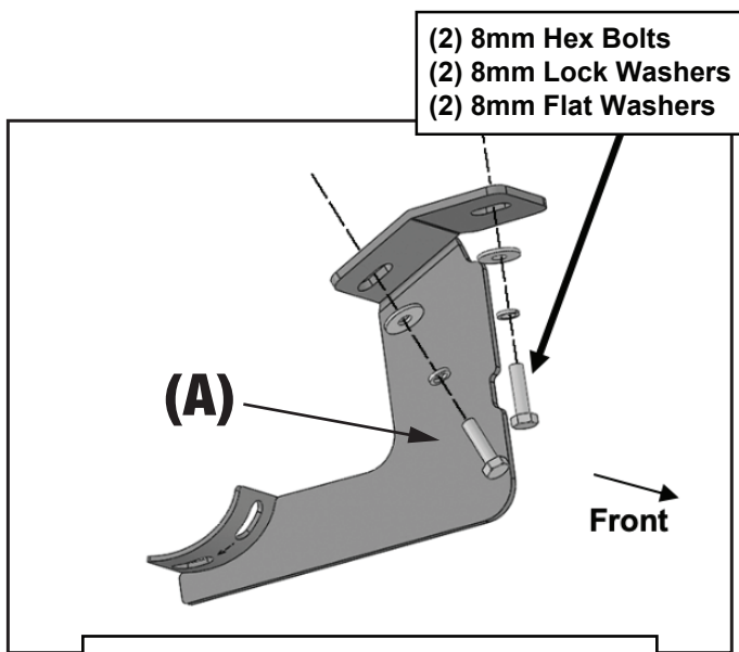
(Fig 3) Attach the Driver/Left Front Mounting Bracket (A) to the front location
