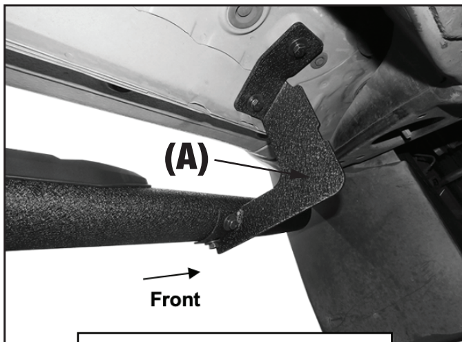
(Fig 8) Driver/Left Sidebar attached to the front Mounting Bracket (A)
