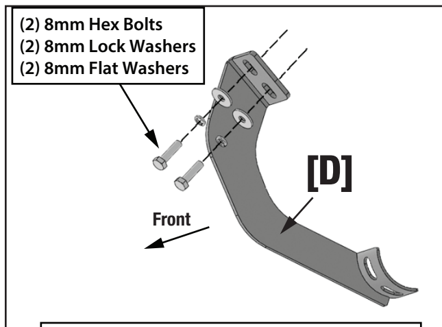
(Fig 5) Attach (1) Passenger/Right Center/Rear Mounting Bracket [D] to the 2nd location
