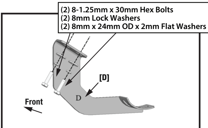
(Fig 7) Attach Passenger/Right Center Mounting Bracket [D] with indicated hardware. DO NOT fully tighten at this time
