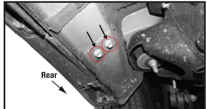
(Fig 9) Locate the Passenger Side Rear mounting location. Remove any plastic tabs or bolts as necessary
