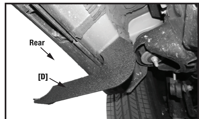
(Fig 12) Attached Passenger/Right Rear Mounting Bracket [D]
