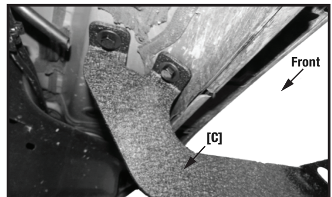
(Fig 4) Attached Passenger/Right Front Mounting Bracket [C]
