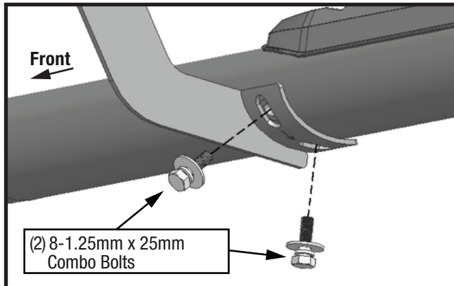
(Fig 13) Use indicated hardware to attach brackets to side bar
