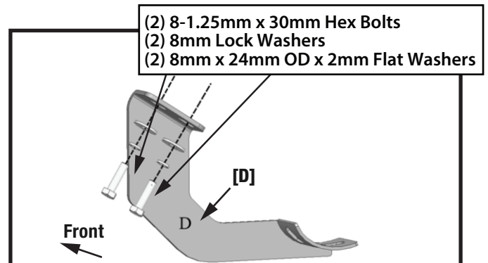
(Fig 11) Attach Passenger/Right Rear Mounting Bracket [D] with indicated hardware. DO NOT fully tighten at this time
