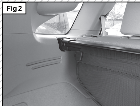
Pull back spring loaded end to fit into pocket
